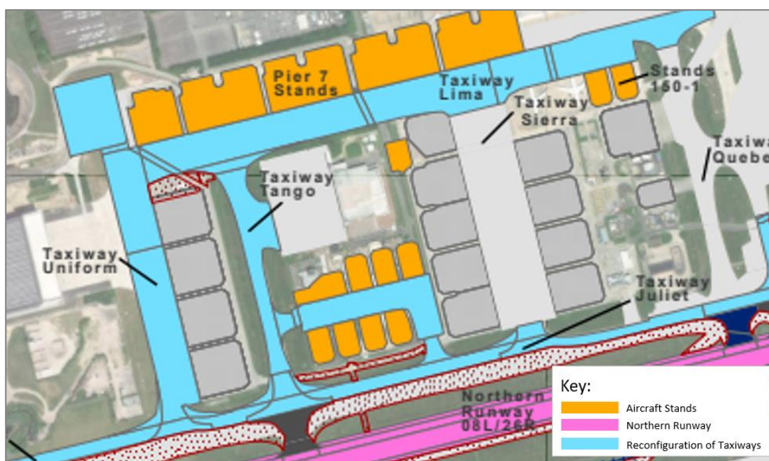
Figure 23: Aircraft stands
